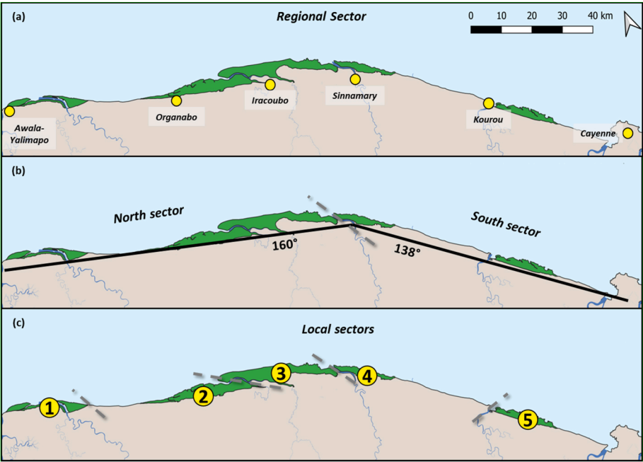
Fig. 6. Geographical sectors used in the MANG@COAST scenarios. (a) Regional sector of approximately 200 km. (b) North and south sectors separated by a grey dashed line where the orientation changes (Sinnamary region). The latter is indicated by the bold black line. (c) Local sectors also separated by grey dashed lines are numbered. Grey dashed lines indicate the boundaries between sectors. They are drawn to follow the orientation of the rivers at their mouths. Mangrove areas are green. Sinnamary is located at 5.39°N and 52.96°W.
